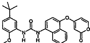
1-(5-tert-Butyl-2-methoxy-phenyl)-3-[4-(2-oxo-2H-pyran-4-yloxy)-naphthalen-1-yl]-urea;
